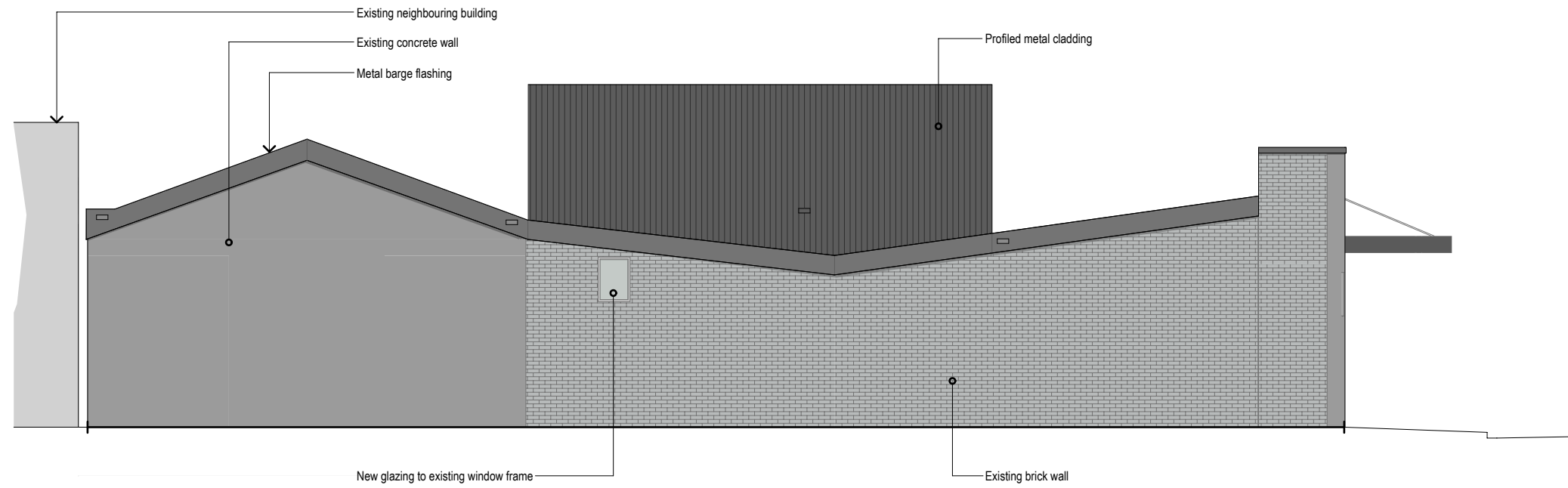
North-East Elevation
