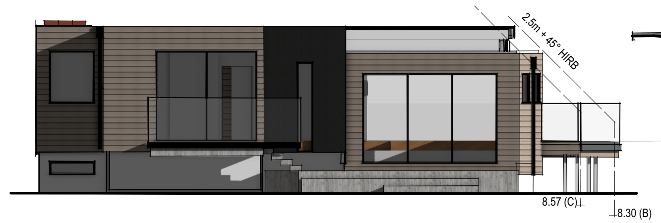
4 south elevation 1:100
