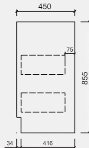
End view
