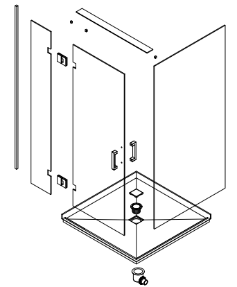
1200x900 2 Wall Hinged System shown
