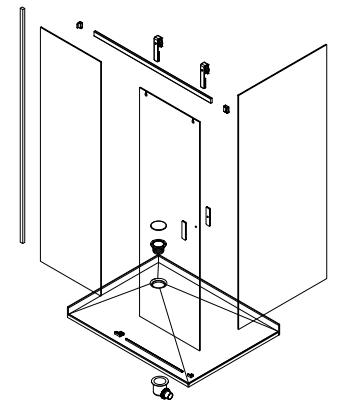
1200x900 2 Wall LH Sliding System shown
