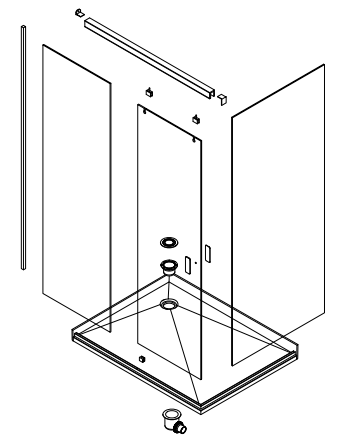
1200x900 2 Wall LH Sliding System shown
