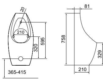
CONTOUR URINAL
