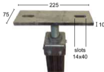
SR-SST Straight Slotted Top
