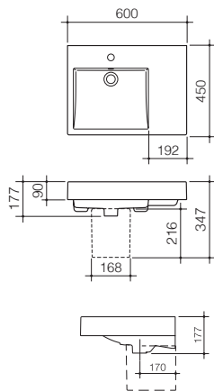
Liano Nexus 600 Wall Basin with Shelf (Right Hand)
