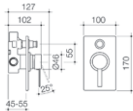
Liano Bath/Shower Mixer with Diverter
