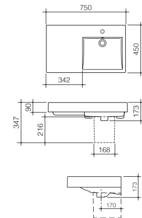
Liano Nexus 750 Wall Basin with Shelf (Left Hand)
