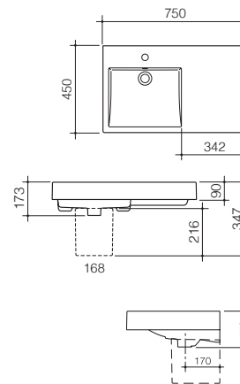
Liano Nexus 750 Wall Basin with Shelf (Right Hand)
