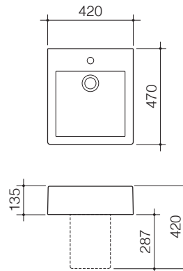
Liano Wall Basin 1 taphole 649315W
