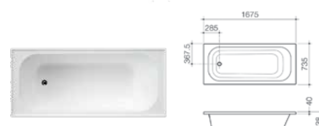
Luna Island Bath
