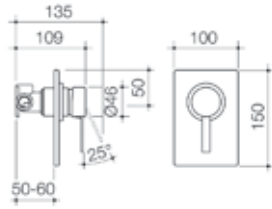
Liano Bath/Shower Mixer with Diverter
