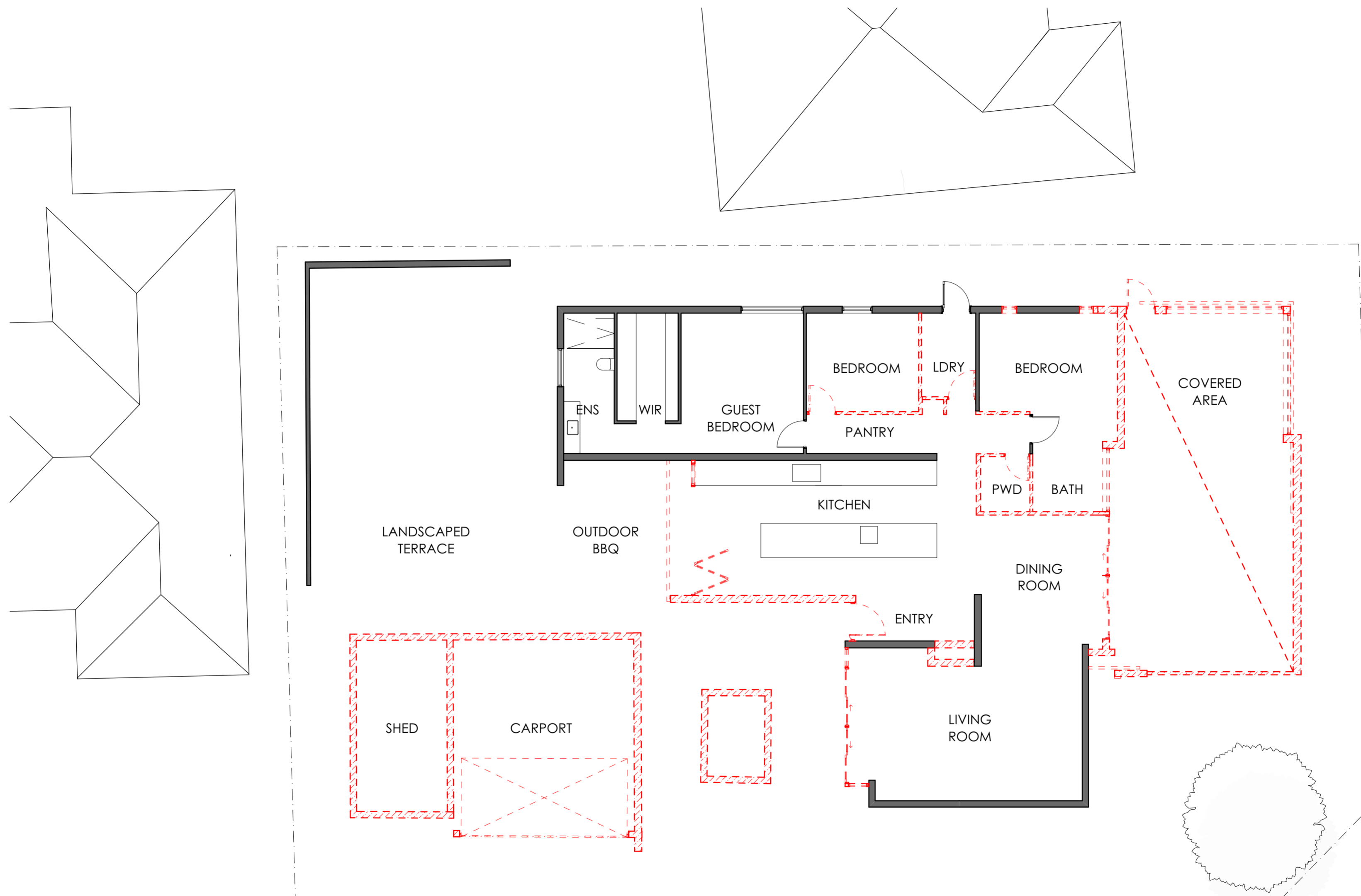
GROUND FLOOR DEMOLITION PLAN
