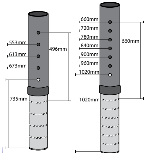
Code 42 Outer: 42mm Dia x 1.6mm RHS Inner: 38mm Dia x 1.6mm RHS Table Height 496 to 735Hmm Counter Height 660mm to 1020mm
