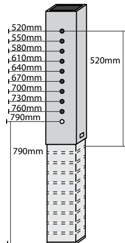
Code 40 Outer: 40mm x 1.6mm SHS Inner: 36mm x 1.6mm SHS 520 to 790Hmm
