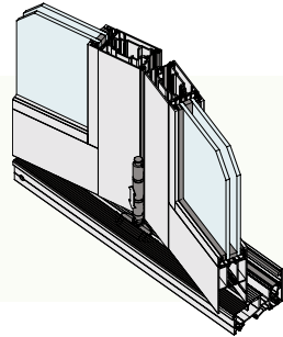
Series 832 Thermally Broken Bi-fold Door (Bottom Rolling)
