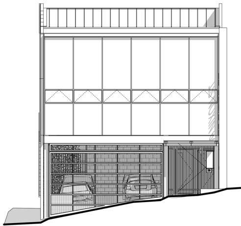
East Elevation
