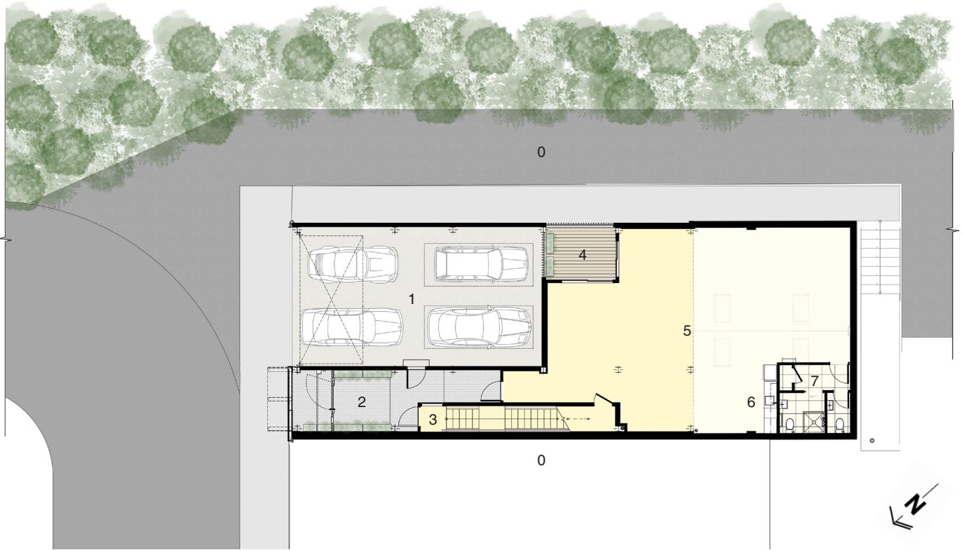
GROUND FLOOR / SITE PLAN
