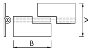
304 Grade Stainless Steel Lift Off Hinge
