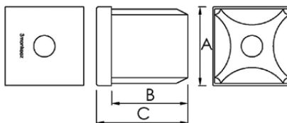
Nylon Leg Insert - Square Tube
