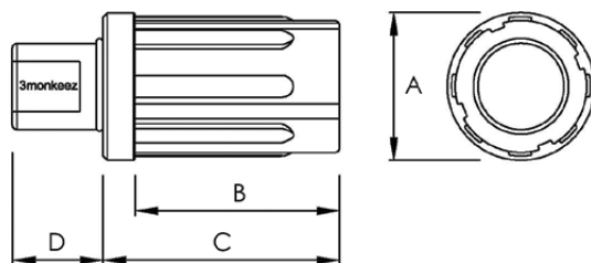
Nylon Adjustable Foot - Round Tube
