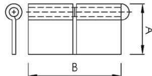
304 Grade Stainless Steel Flag Hinge
