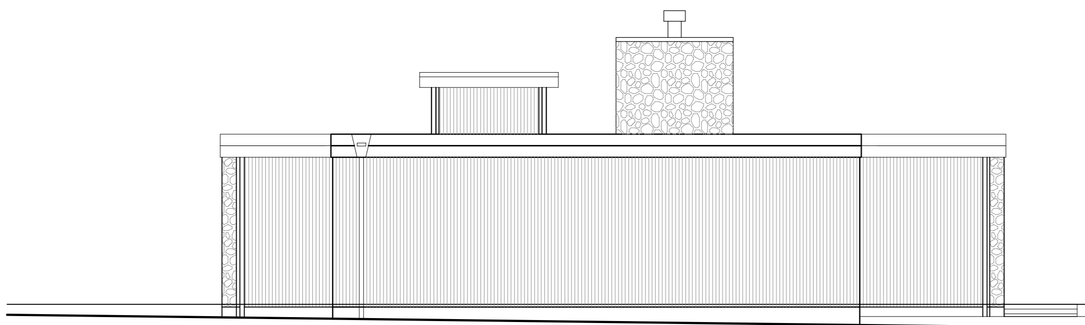
south elevation
