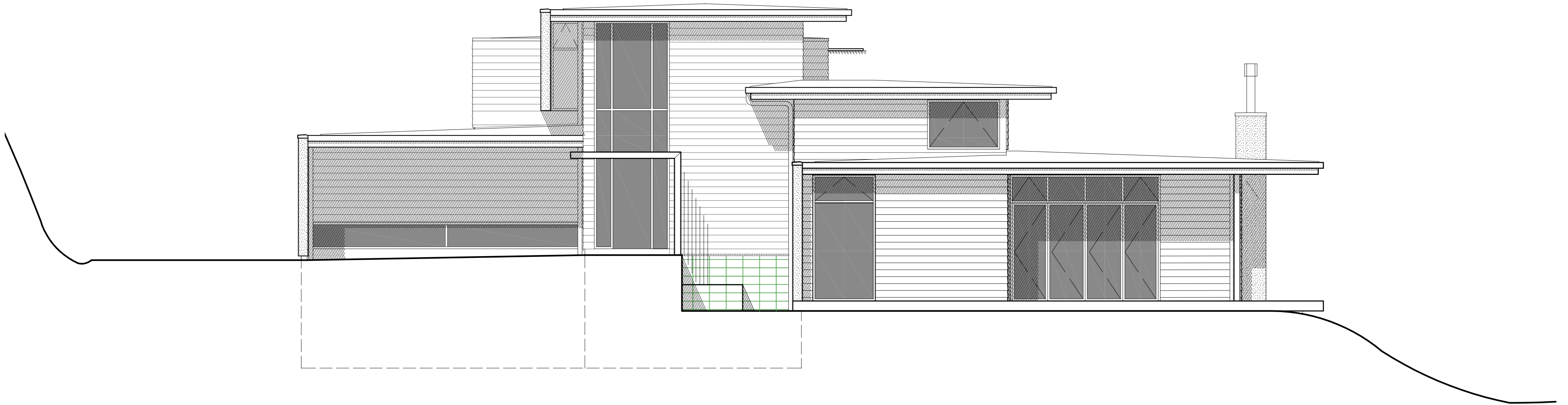
east elevation
