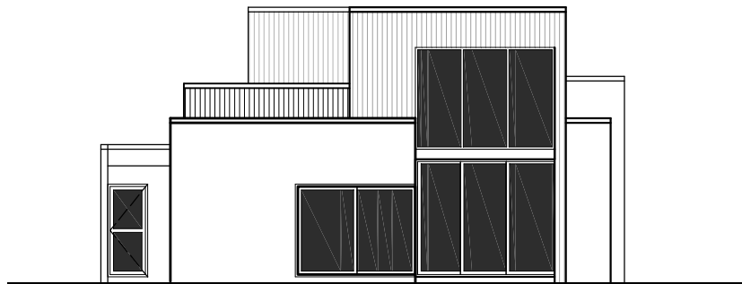
south elevation
