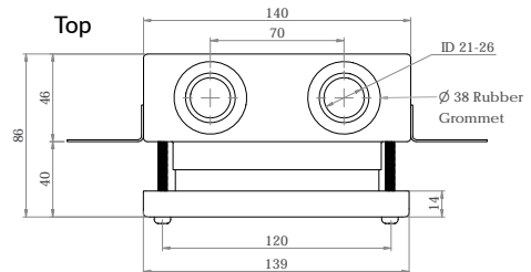
Cross Section
