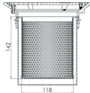
Cross Section
