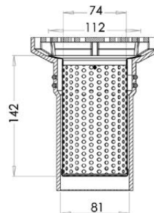
Cross Section
