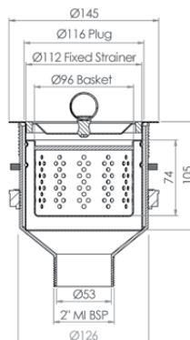
Cross Section
