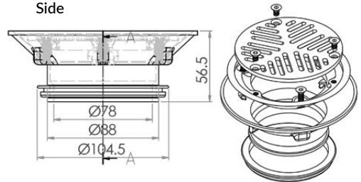
Side
