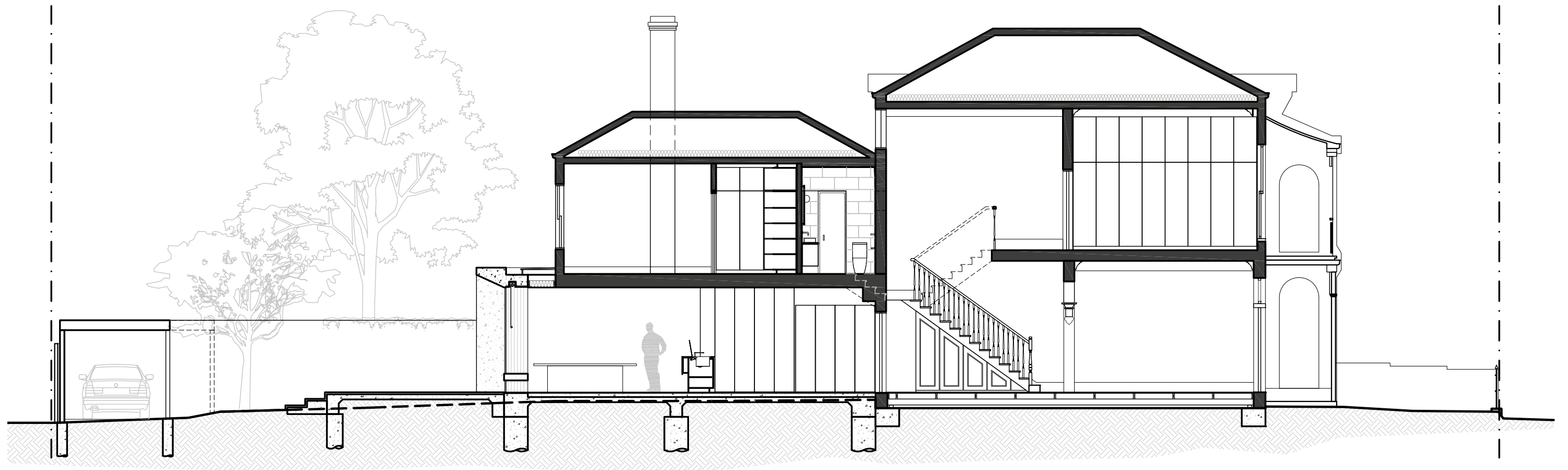
Section A
