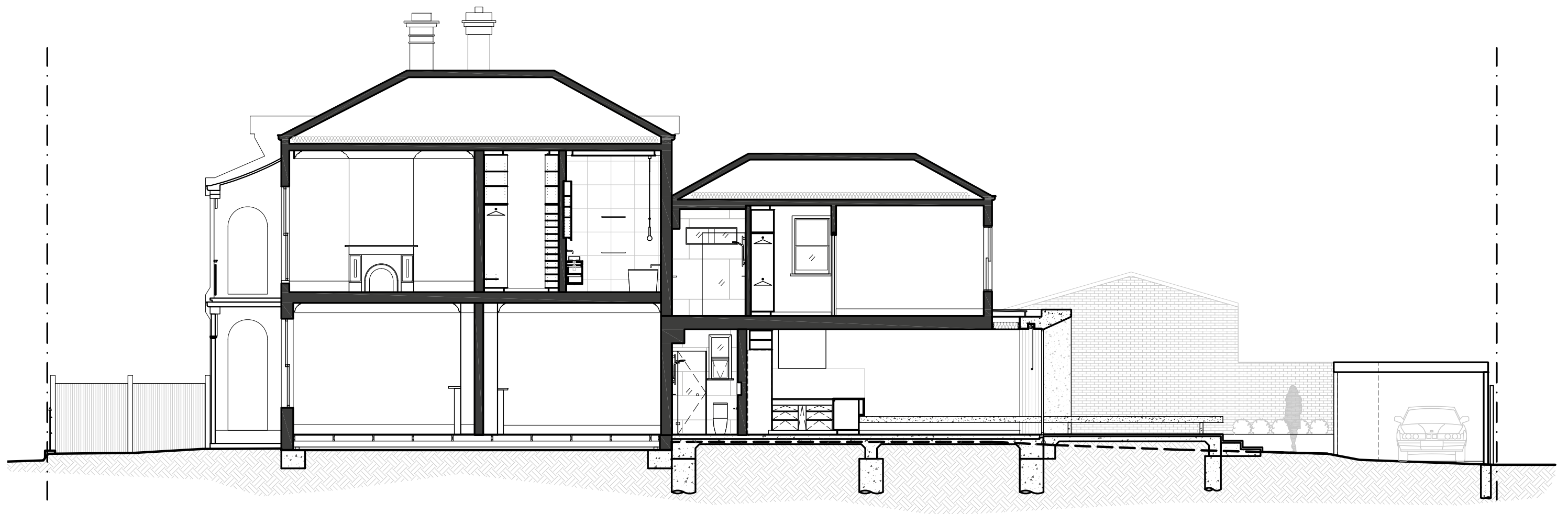
Section B
