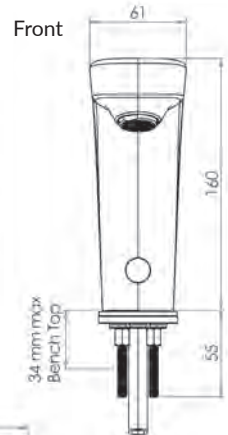
Solenoid Unit
